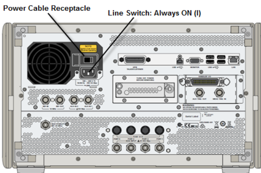
Figure 2 Line switch (Always ON) and power cable receptacle
